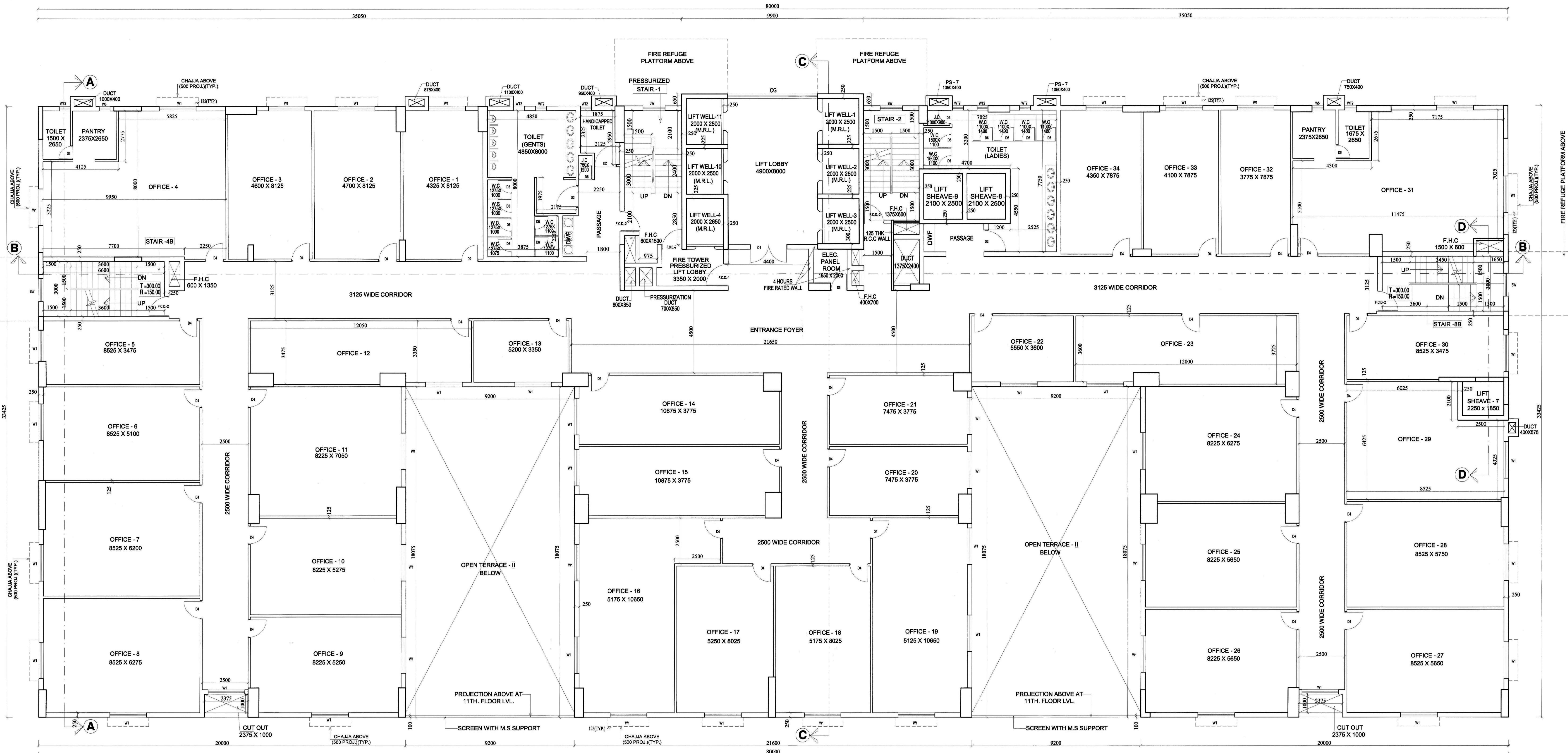
THIRD FLOOR PLAN (14.7 M. LVL. OF FLOOR) SCALE: 1:100
